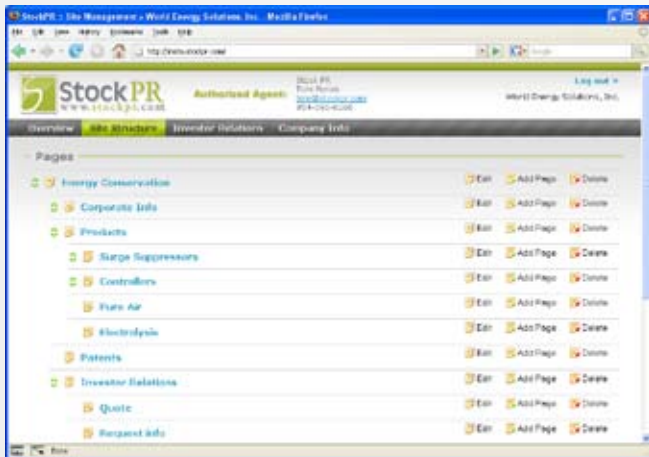
Site Structure
